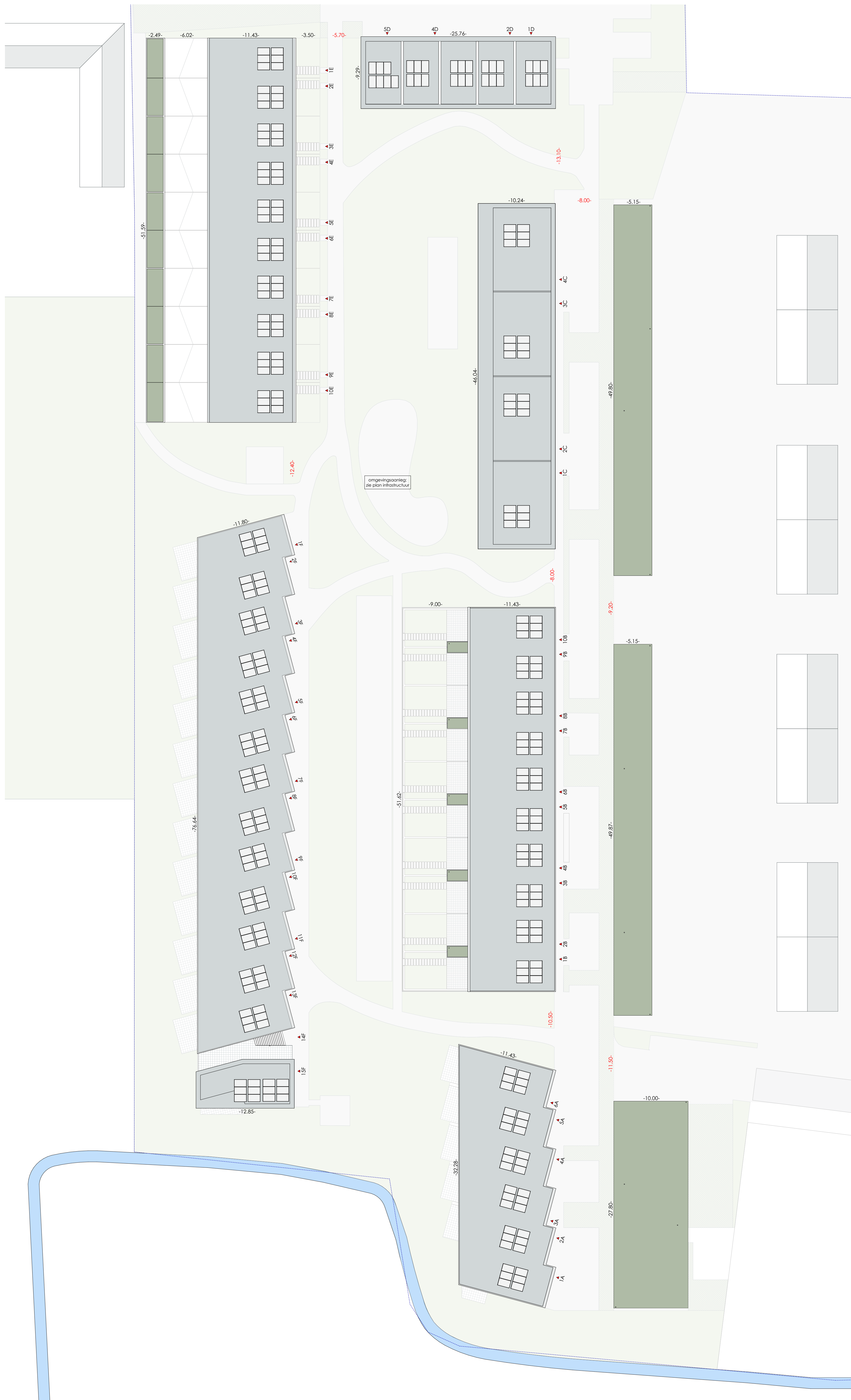
Schema inplanting 1/1000
